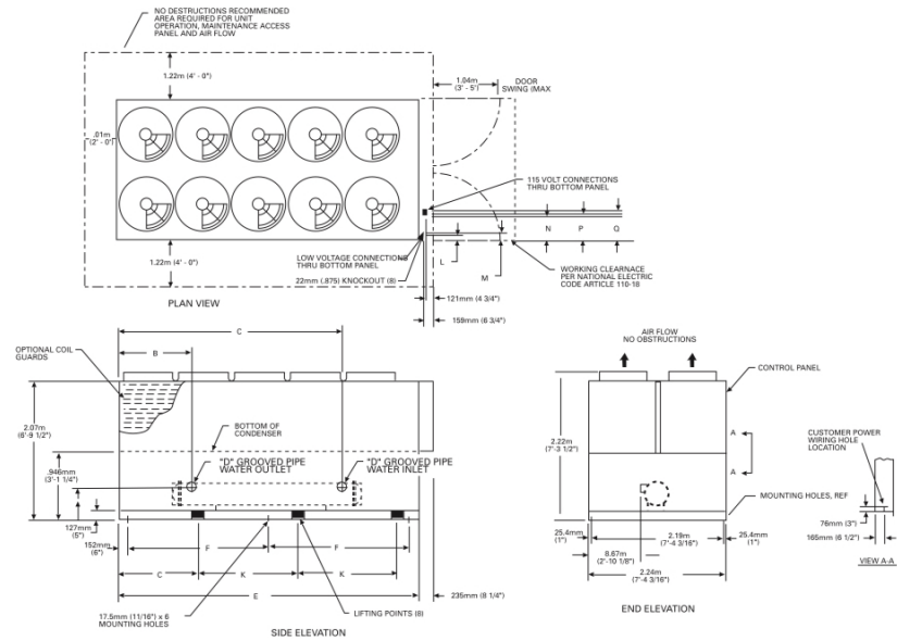
Figure D-1 — RTAA 70-125 Unit Dimensions
