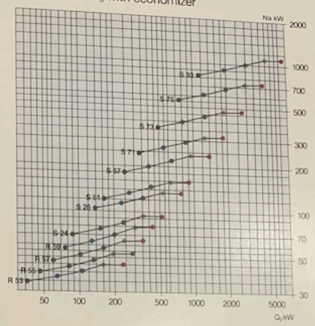
Refrigerant R22 with economizer
