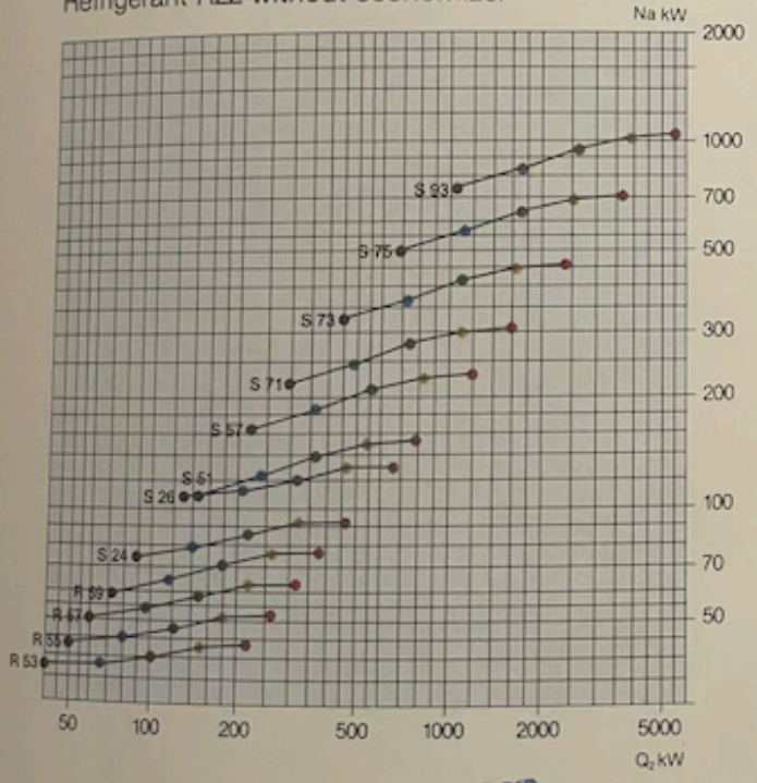
Refrigerant R22 without economizer
